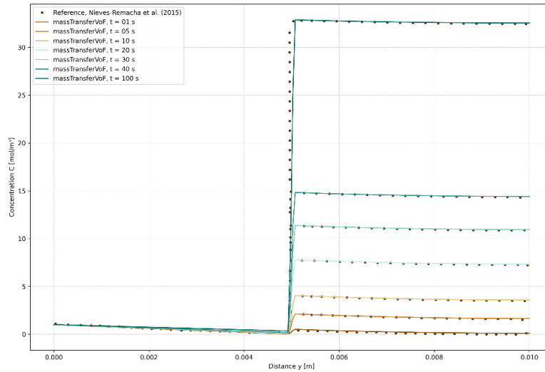
Figure 4. Case 3 – Reference (Nieves-Remacha et al., 2015) and OpenFOAM solution produce similar results during mass transfer and tracer spreading for D_L = 10^{-5} \text{ m}^2/\text{s} and D_G = 10^{-5} \text{ m}^2/\text{s} , illustrating the accuracy of the algorithm, illustrated times: 1 s, 5 s, 10 s, 20 s, 30 s, 40 s, 100 s.
