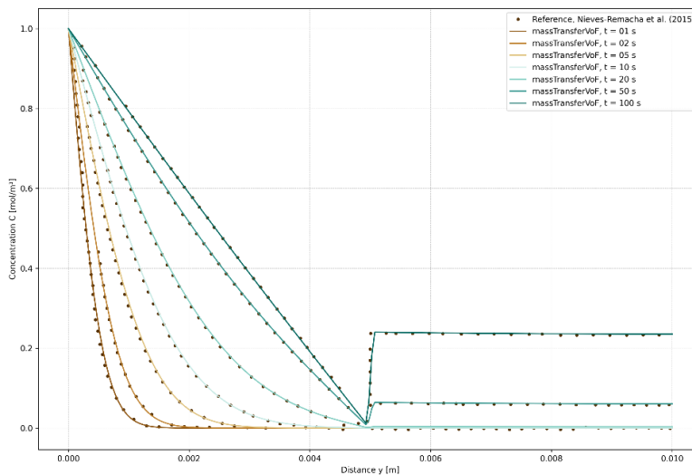
Figure 5. Case 3 – Reference (Nieves-Remacha et al., 2015) and OpenFOAM solution produce similar results during mass transfer and tracer spreading for D_L = 10^{-7} \text{ m}^2/\text{s} and D_G = 10^{-5} \text{ m}^2/\text{s} , illustrating the accuracy of the algorithm, illustrated times: 1 s, 2 s, 5 s, 10 s, 20 s, 50 s, 100 s.
